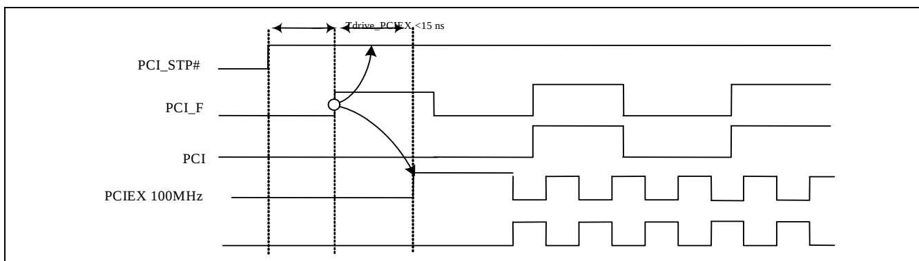
Figure 8. PCI_STP# Deassertion
