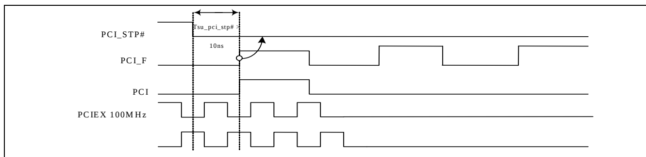
Figure 7. PCI_STP# Assertion
