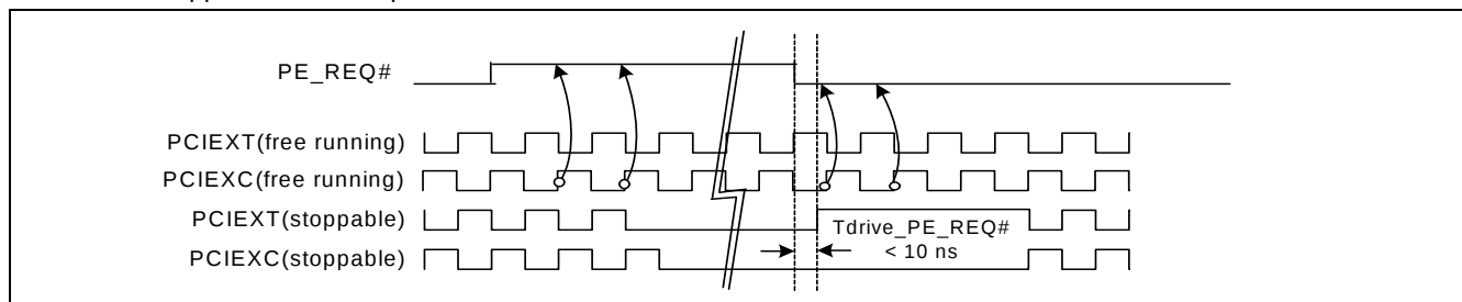
Figure 9. CLKREQ# Deassertion
