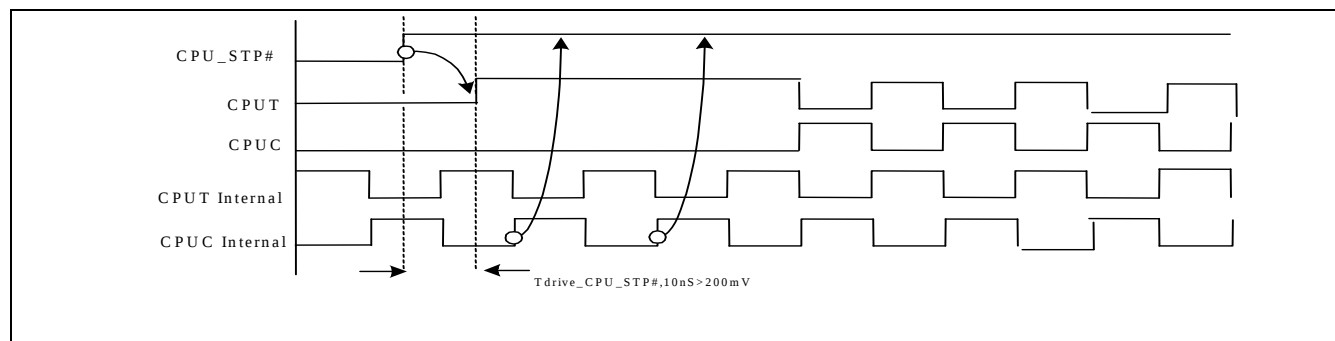
Figure 6. CPU_STP# Deassertion
